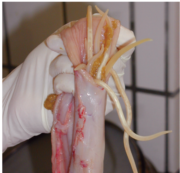
Figure 11: Small intestinal infection with Parascaris spp.
